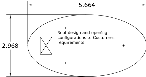
ROOF PLAN
